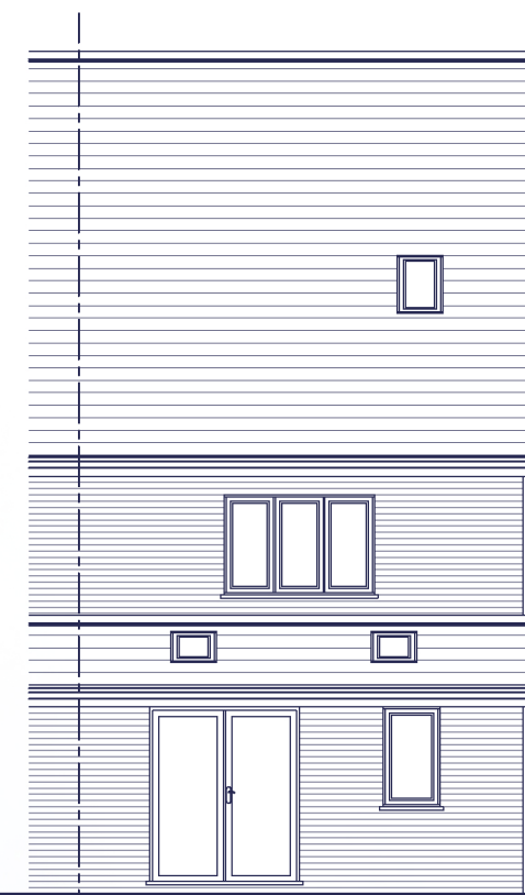
REAR ELEVATION
