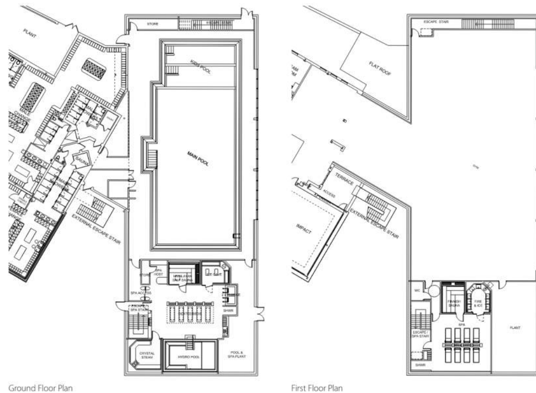
Figure 4: Proposed ground and first floor plan.
