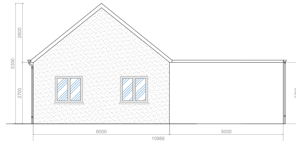
Left Elevation
