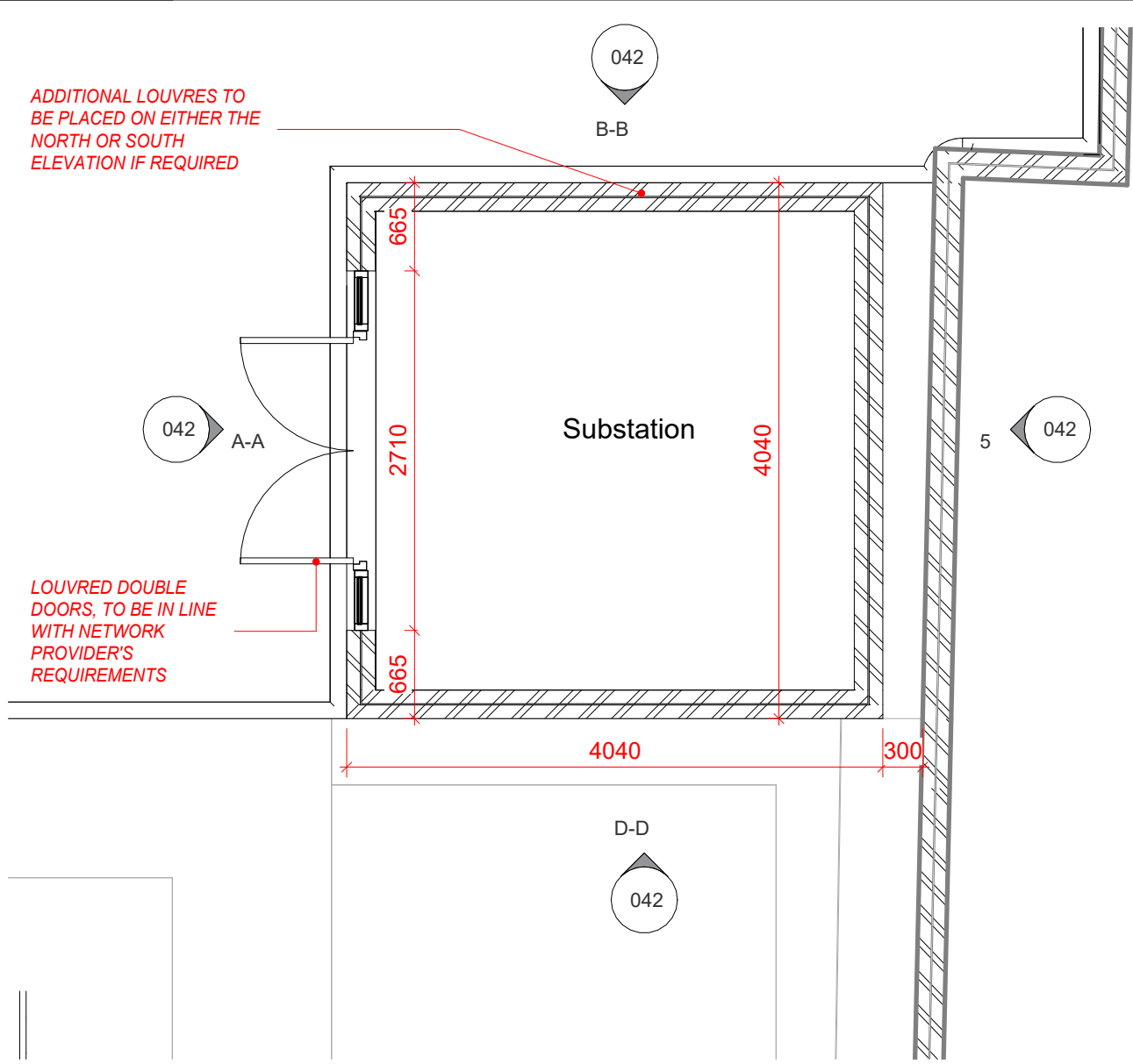
Substation Plan 1 : 50
