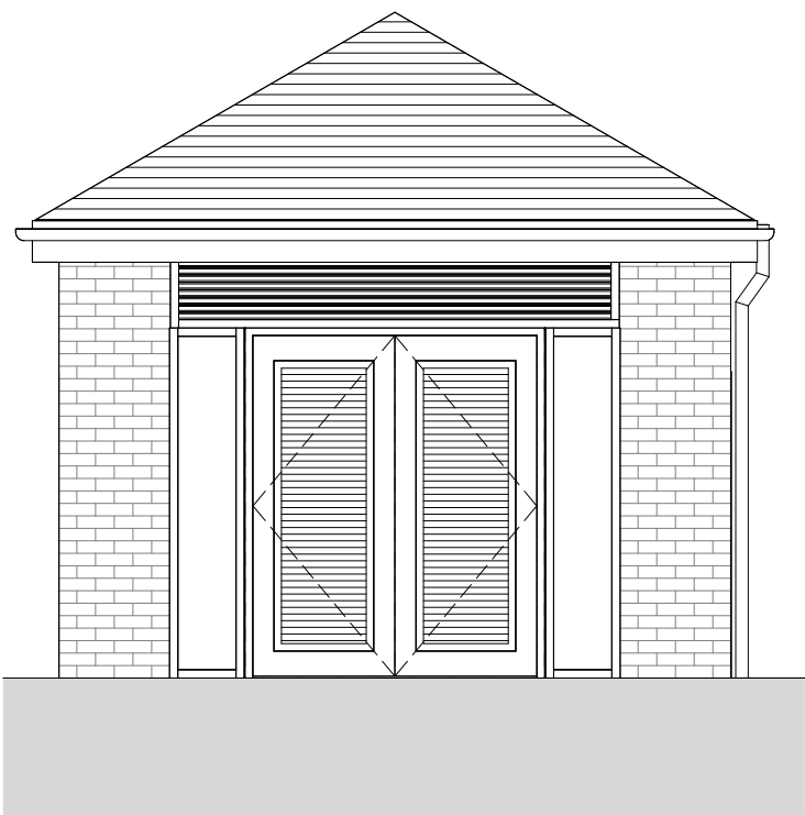
Substation - Elevation A-A 1 : 50
