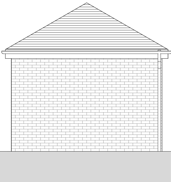
Substation - Elevation D-D 1 : 50
