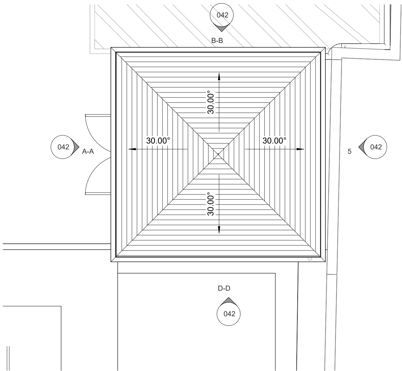
Substation Plan - Roof 1 : 50
