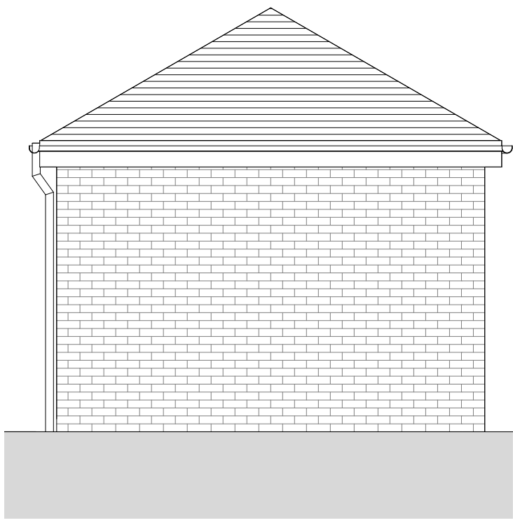
Substation - Elevation C-C 1 : 50
