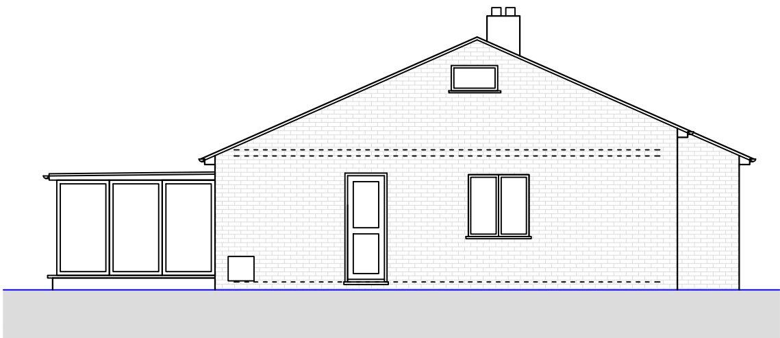
○ Side Elevation 2 1:100
