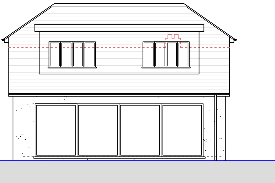
○ Rear Elevation 1 : 1 0 0
