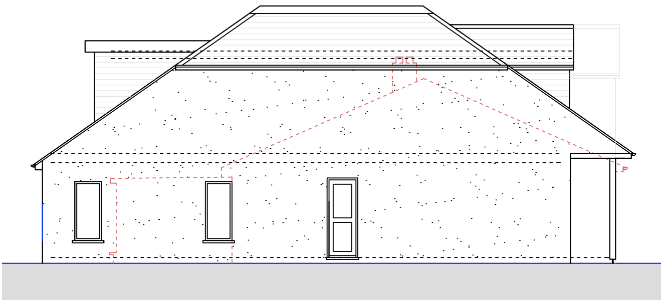
○ Side Elevation 1 1 : 1 0 0
