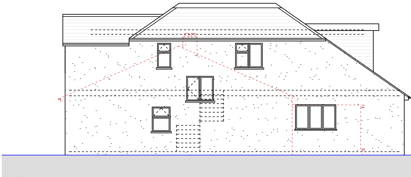
○ Side Elevation 2 1 : 1 0 0
