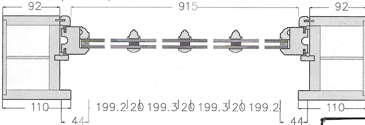
Section C2 (scale 1:4)
