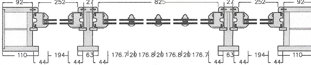
Section C1 (scale 1:4)
