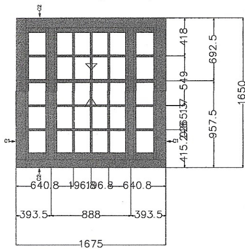
View from outside (scale 1:25)
