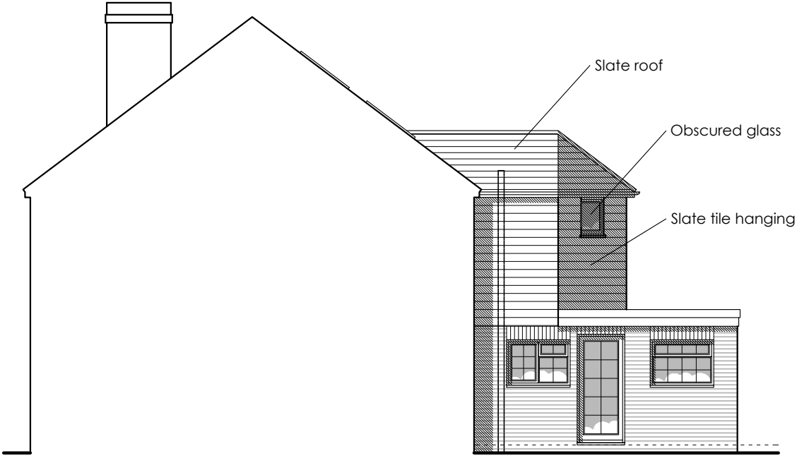
SIDE ELEVATION 1:100
