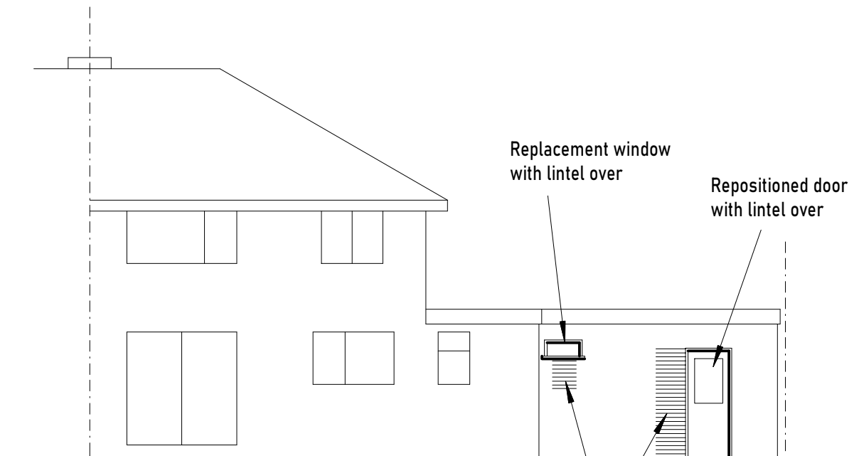
REAR
