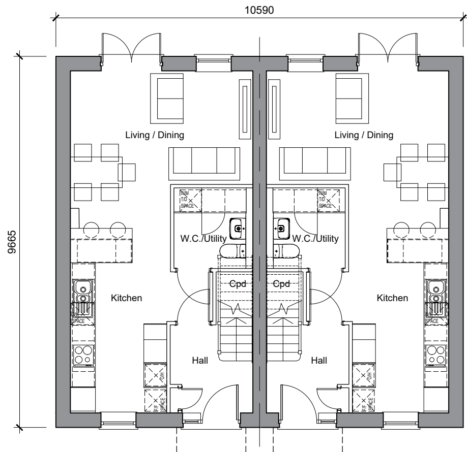
PH3D - 3 Bedroom House NA 113.82sqm
