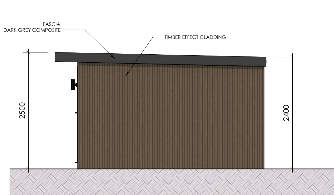
SIDE ELEVATION - S/W
