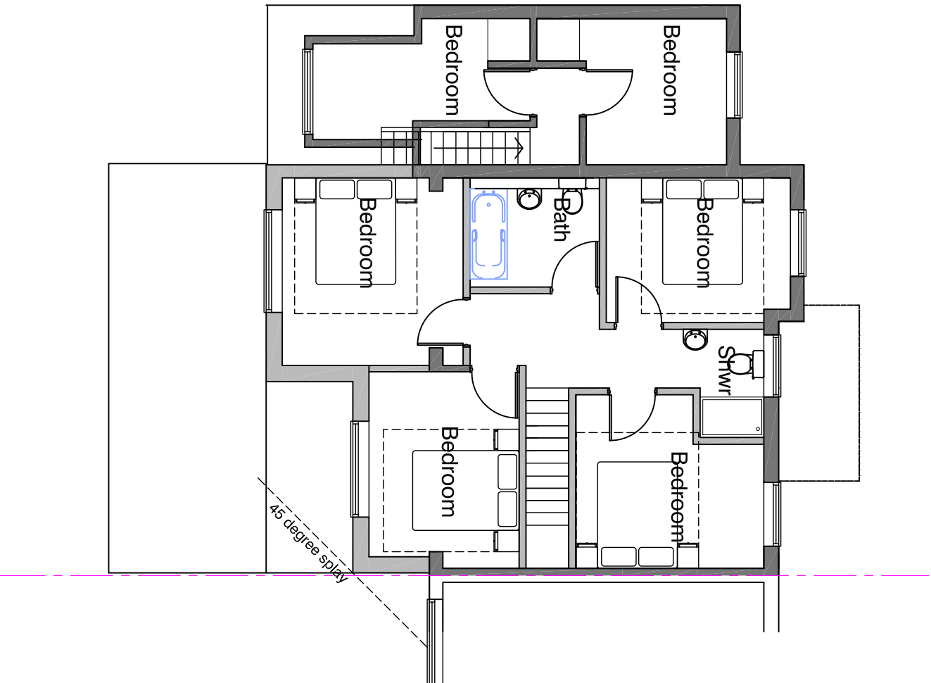
First Floor Plan P R O P O S E D
