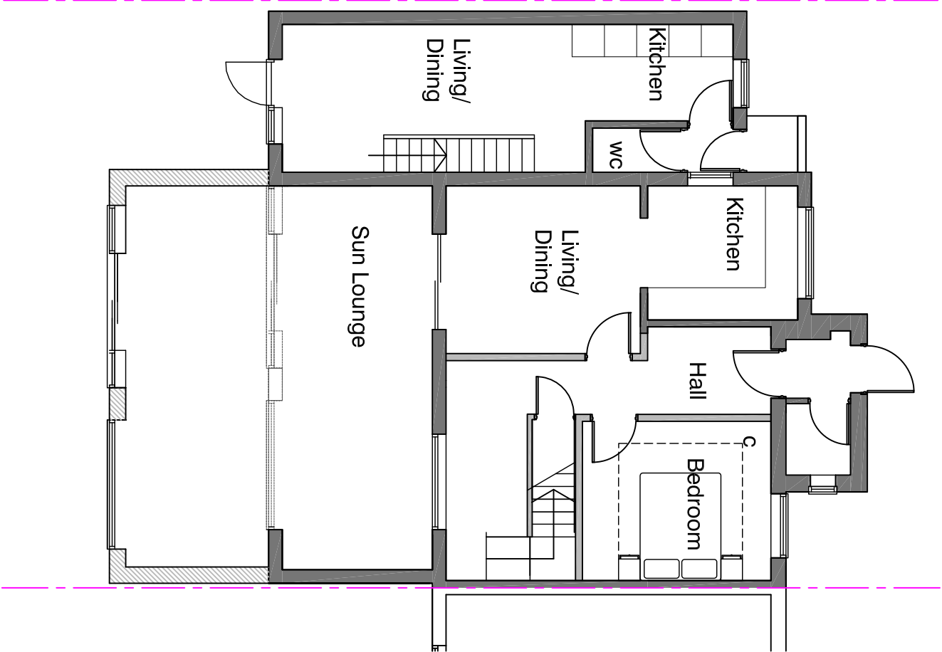
Ground Floor Plan P R O P O S E D
