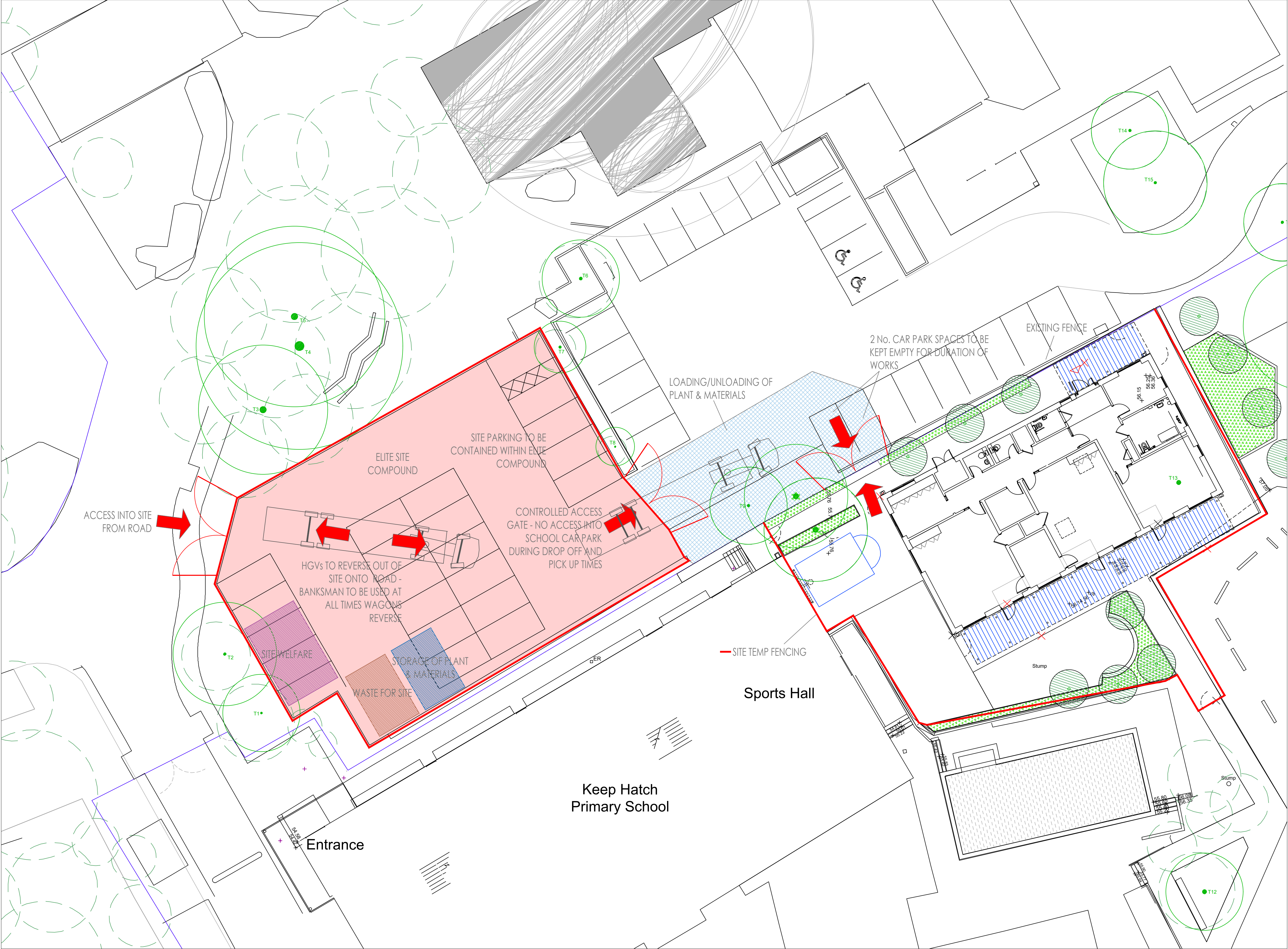
Site Access Plan @ 1:250
