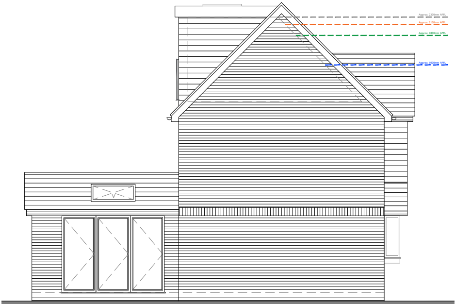
Side Elevation
