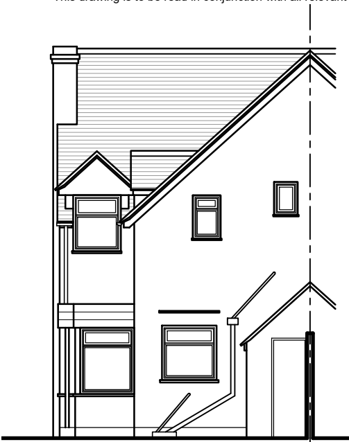
NORTH-EAST ELEVATION
