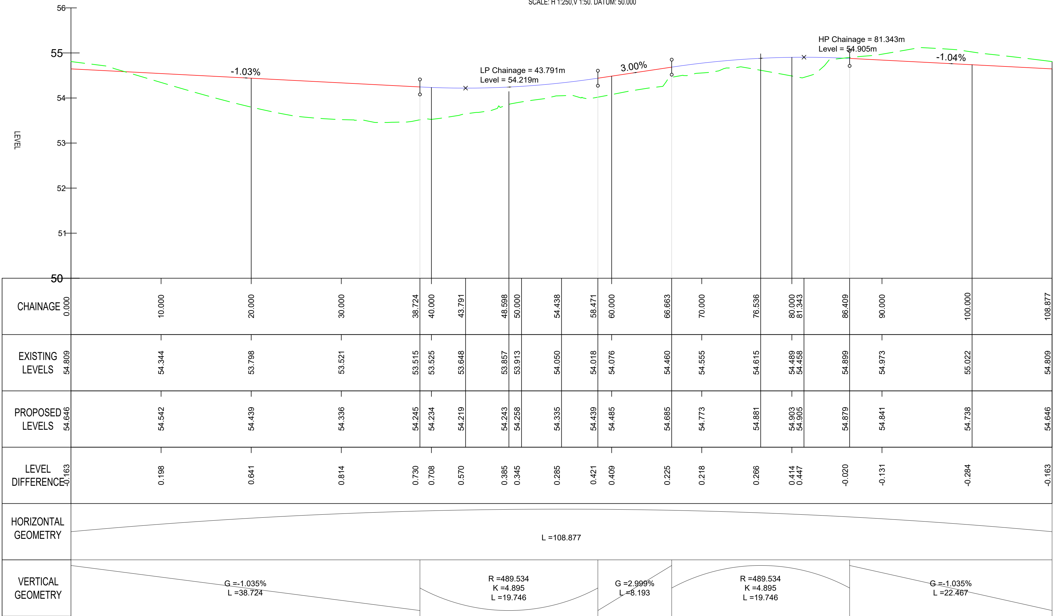
CIRCULATORY CROWN LONGSECTION (M004)
