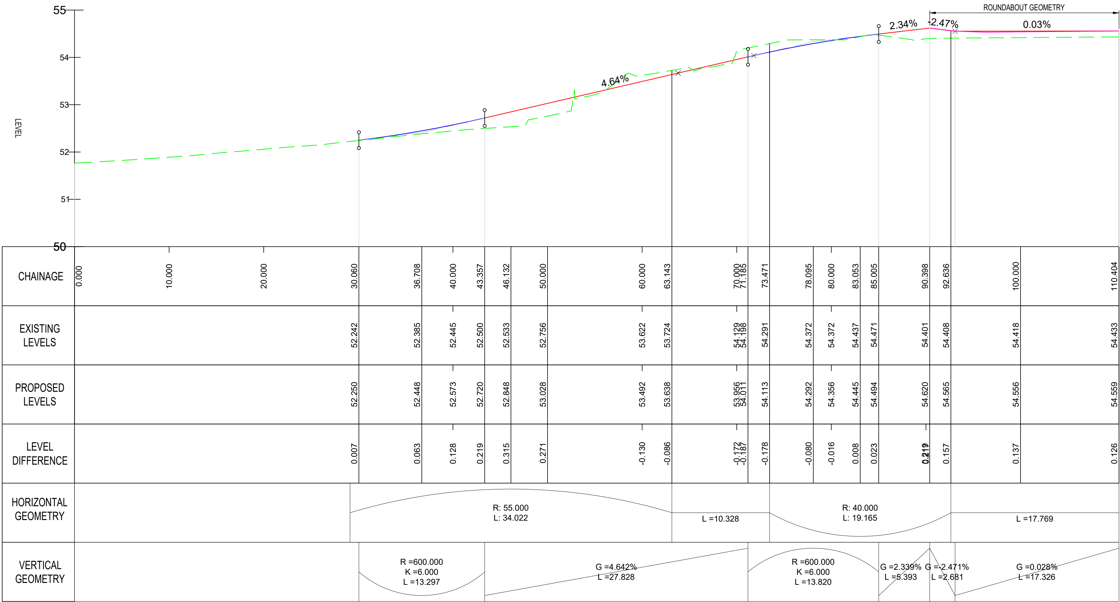
MOLLY MILLARS LANE LONGSECTION (M003)
