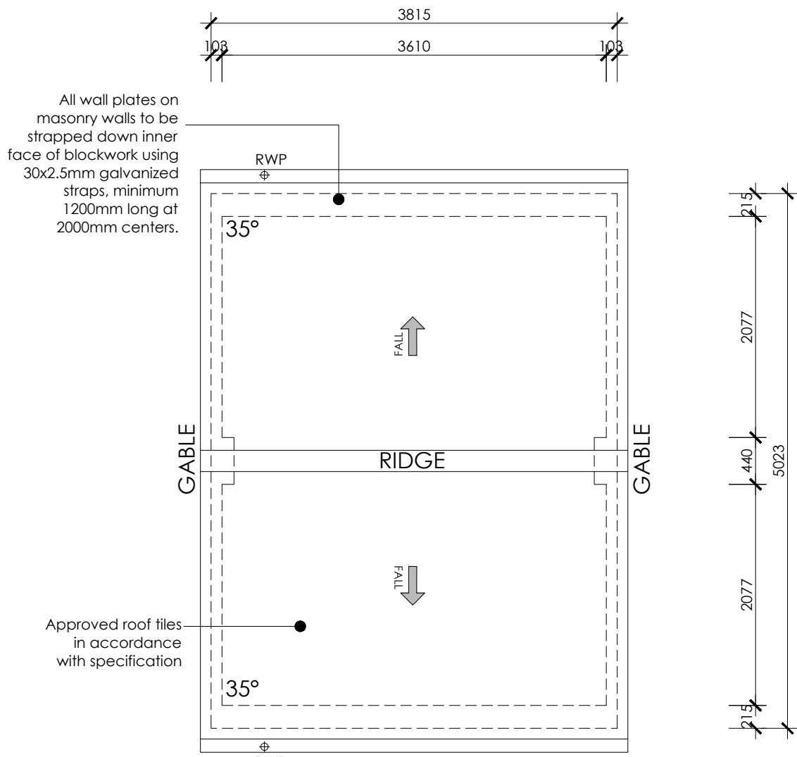
CYCLE STORE ROOF PLAN
