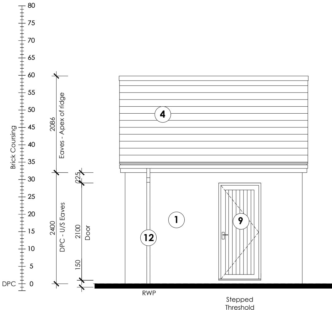
CYCLE STORE FRONT ELEVATION
