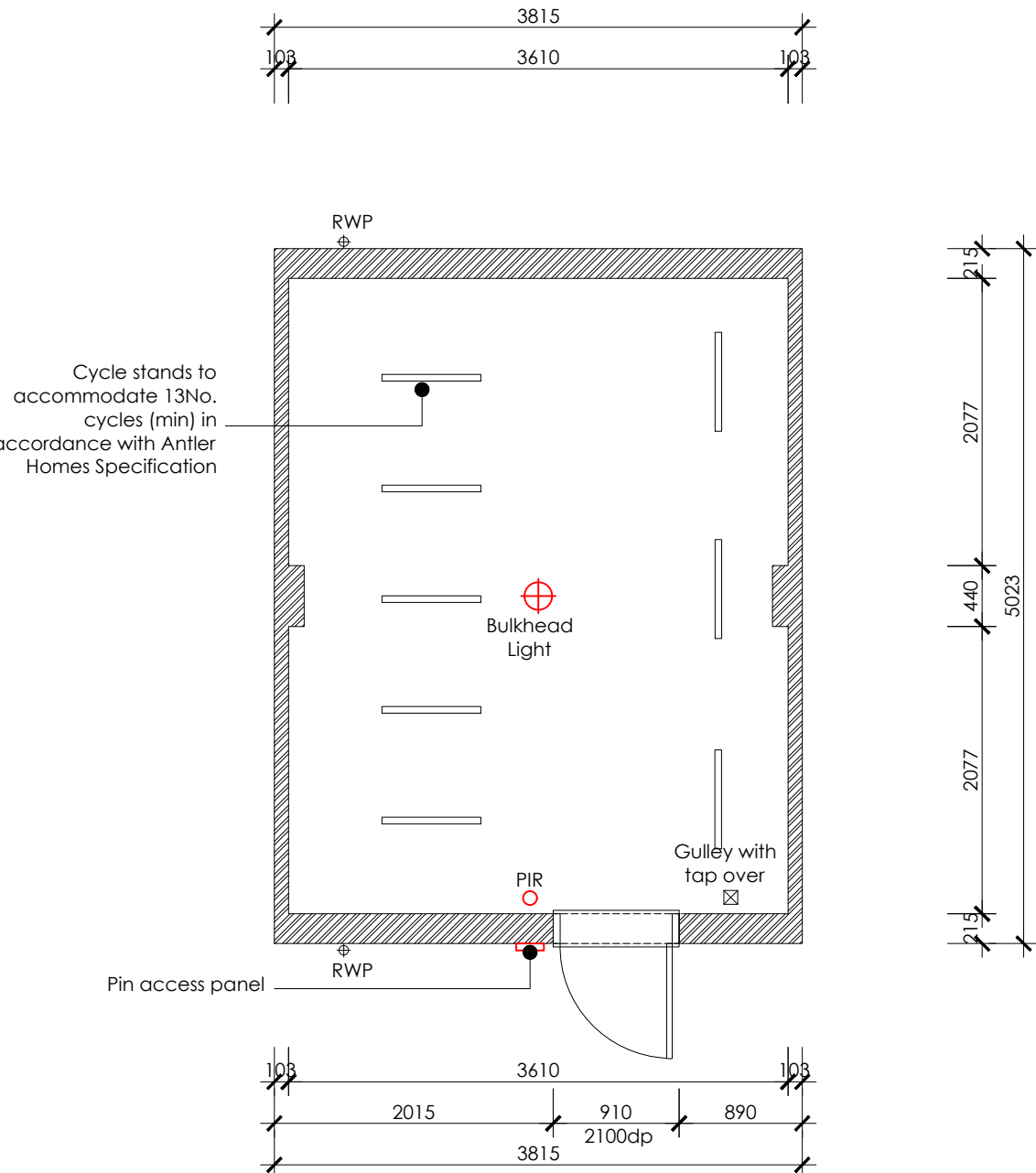
CYCLE STORE FLOOR PLAN
