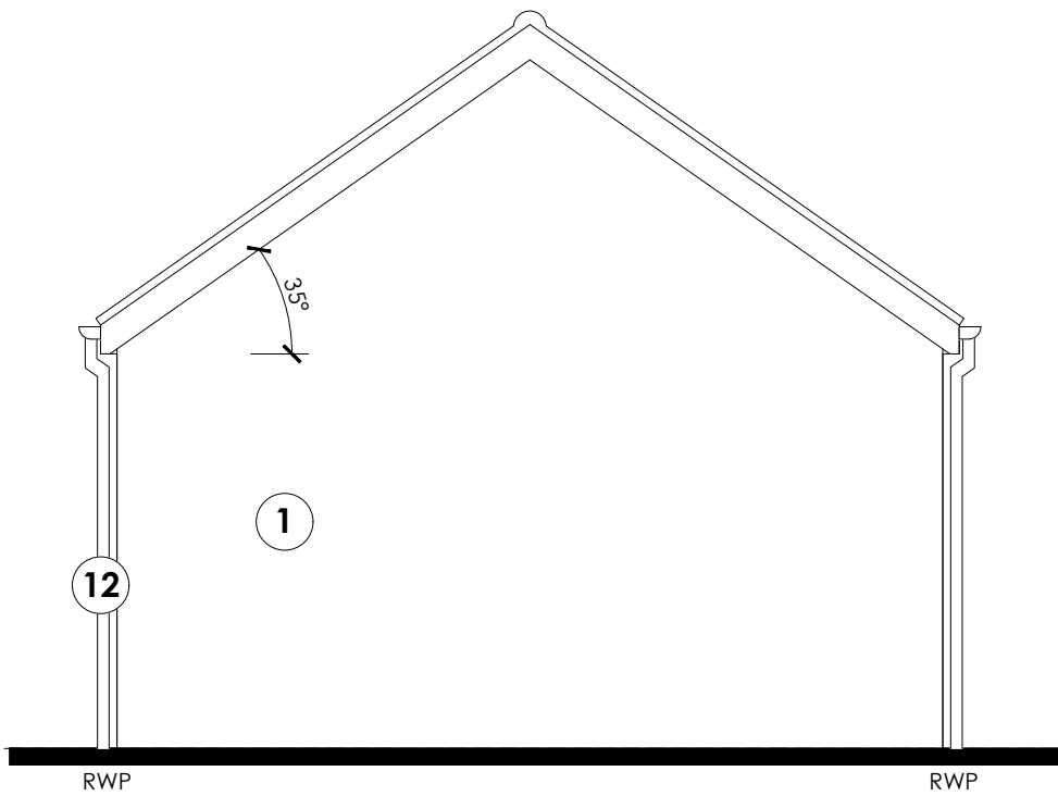
CYCLE STORE SIDE ELEVATION
