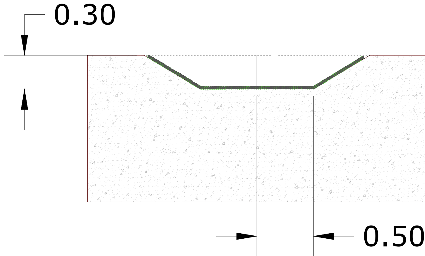
Swale Section
