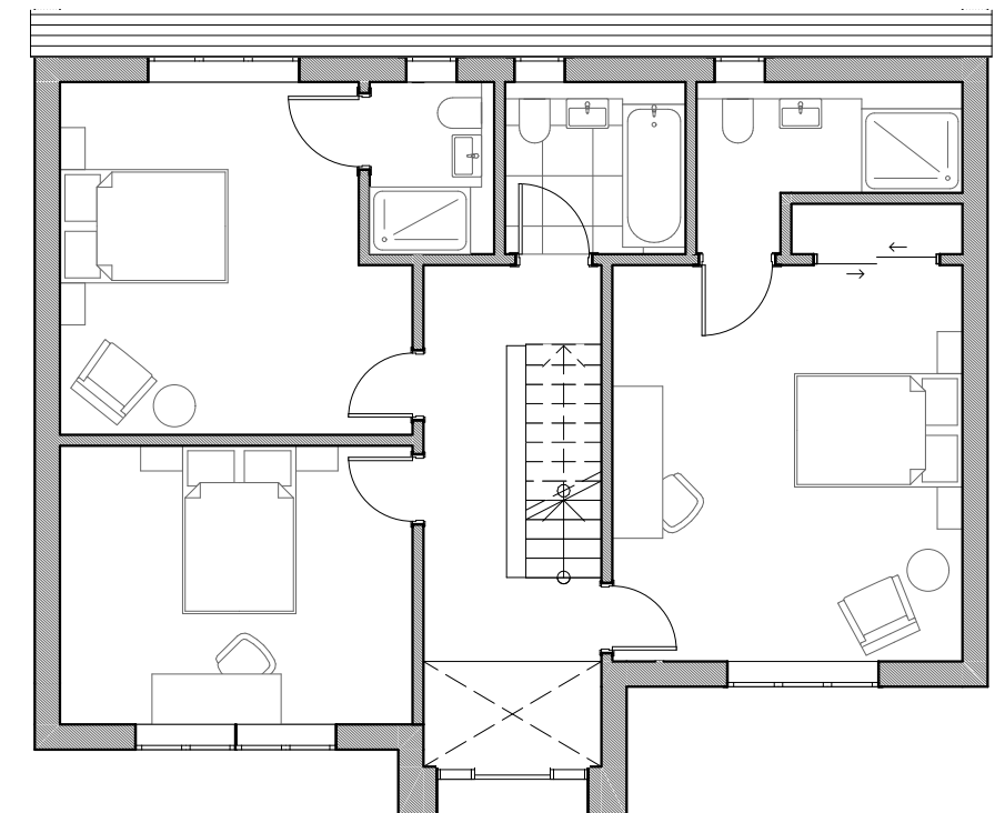
PROPOSED FIRST FLOOR PLAN 1:100 Land North of Oakview, Mill Lane, Wokingham RG41 5DF
