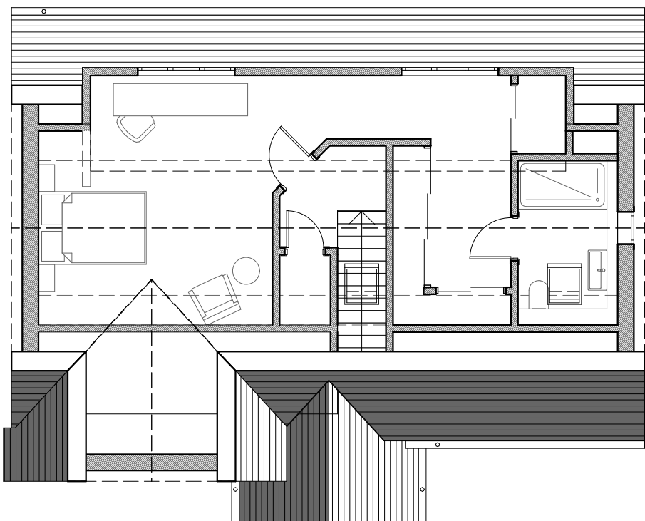
PROPOSED SECOND FLOOR PLAN 1:100 Land North of Oakview, Mill Lane, Wokingham RG41 5DF
