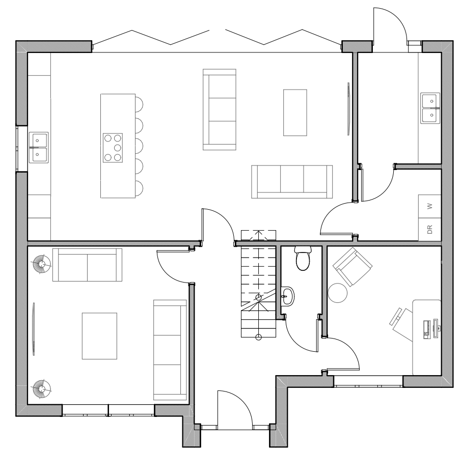
PROPOSED GROUND FLOOR PLAN 1:100 Land North of Oakview, Mill Lane, Wokingham RG41 5DF
