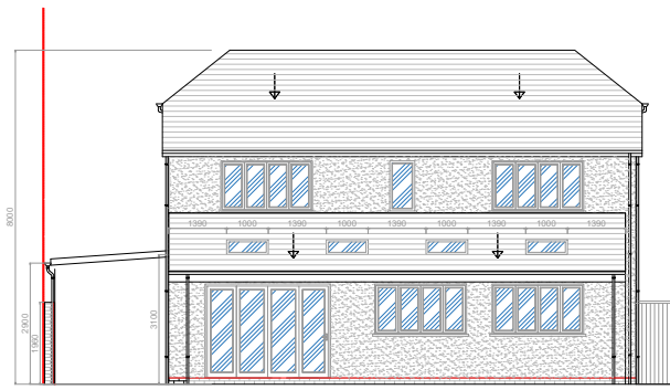
Rear Elevation
