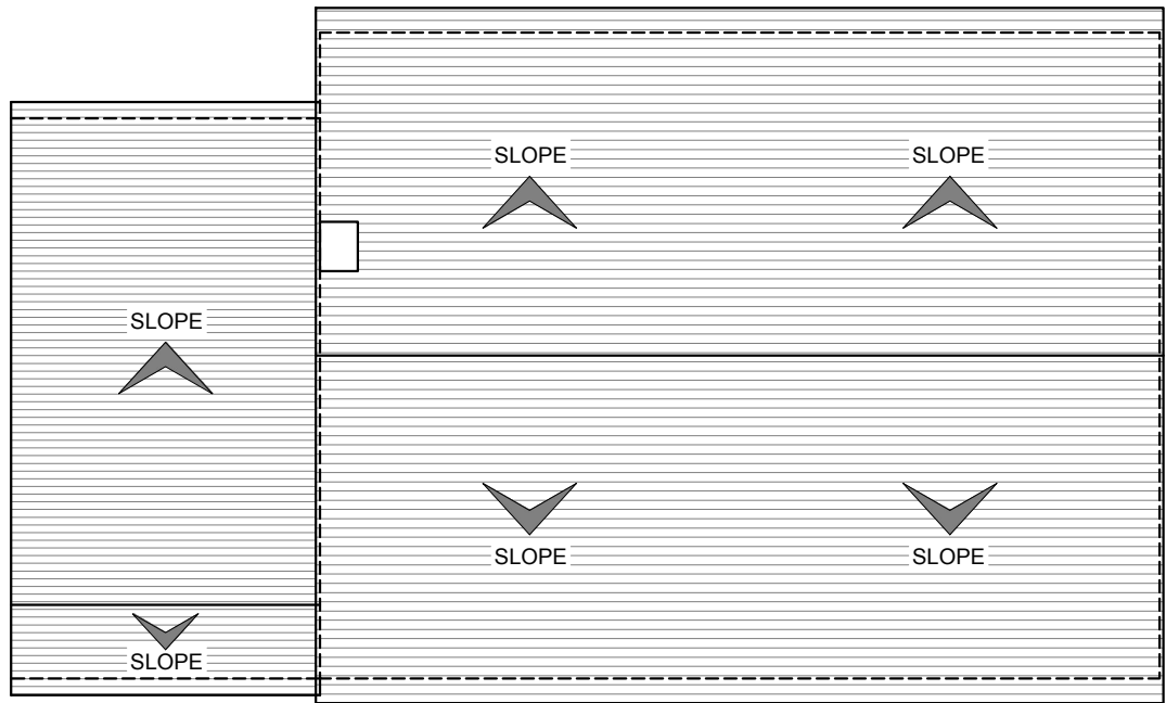
EXISTING ROOF PLAN SCALE= 1:100
