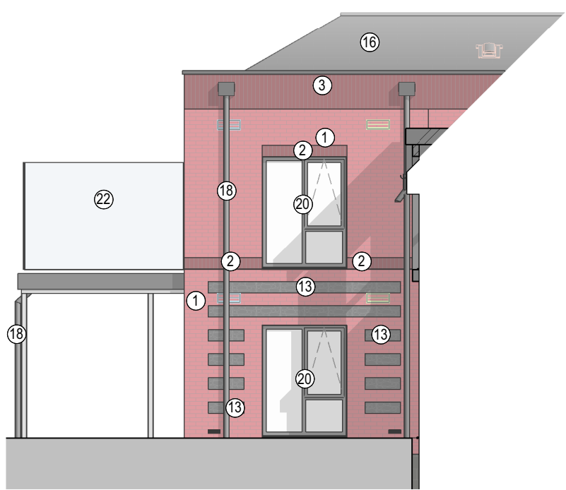
West Elevation (hidden) planning 1:100
