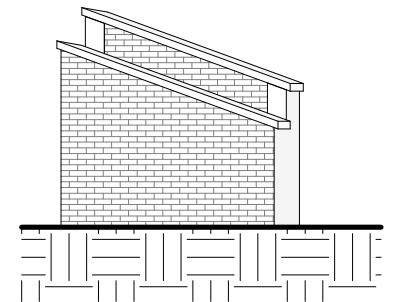
Sections G
