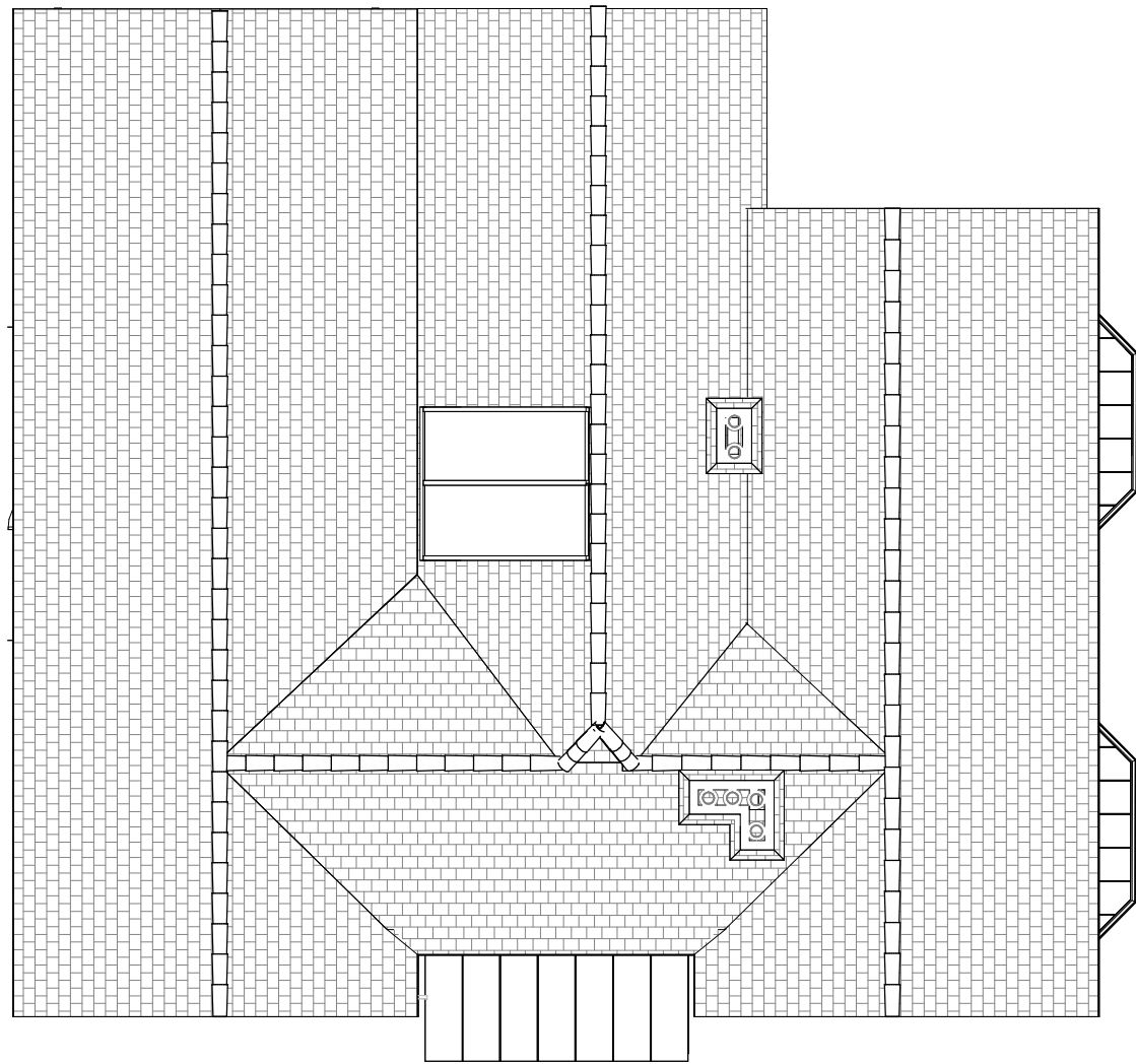
Roof Plan
