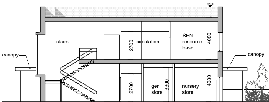
SECTION E
