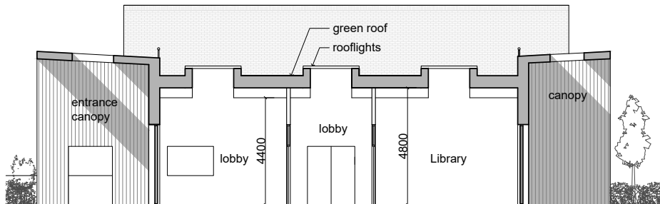
SECTION D
