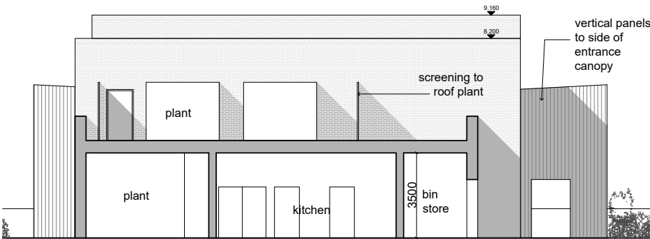
SECTION B
