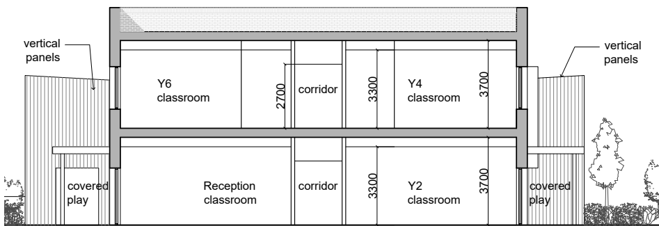
SECTION F
