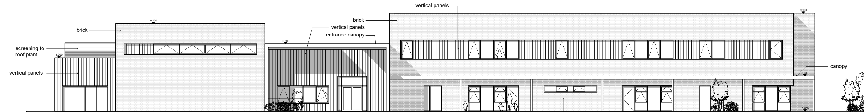
SOUTH ELEVATION
