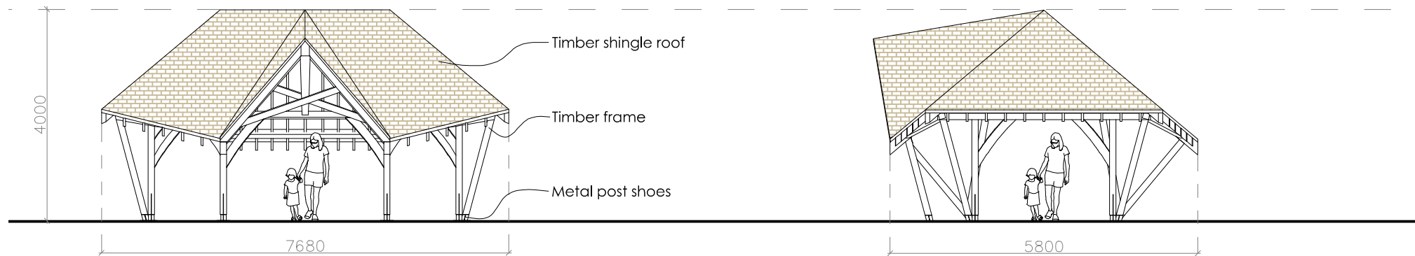
South East Elevation (Front)
