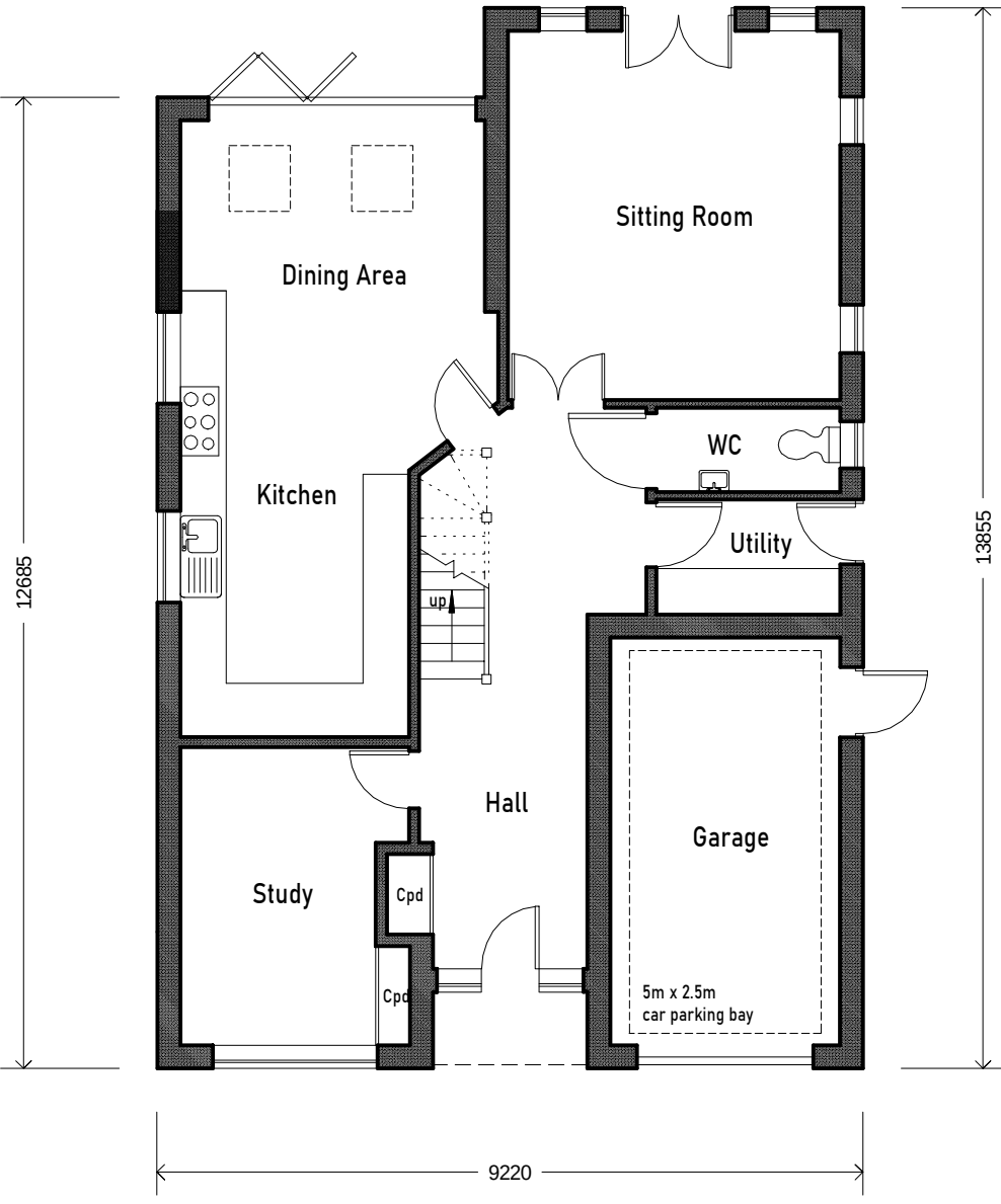
GROUND FLOOR
