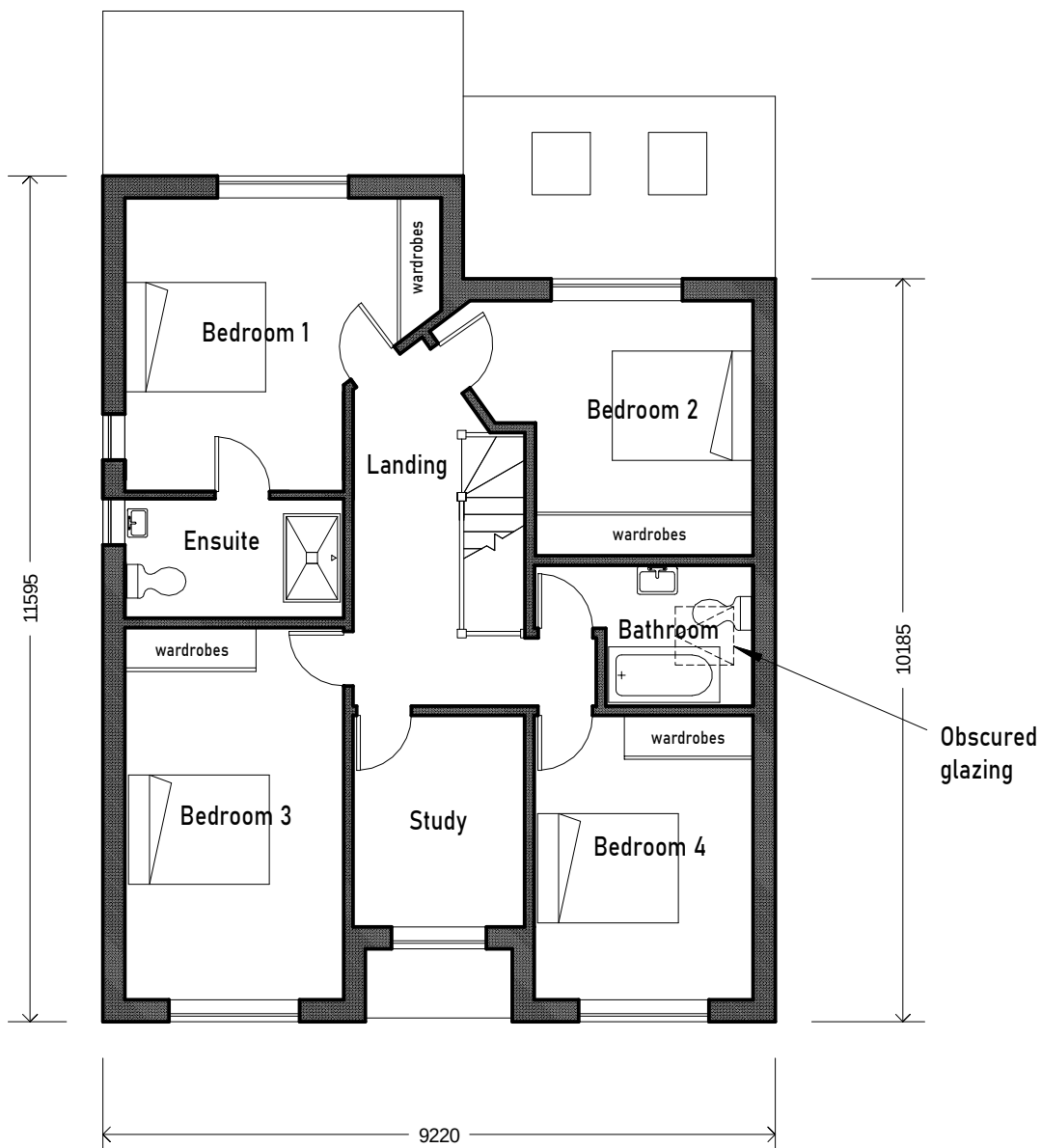
FIRST FLOOR
