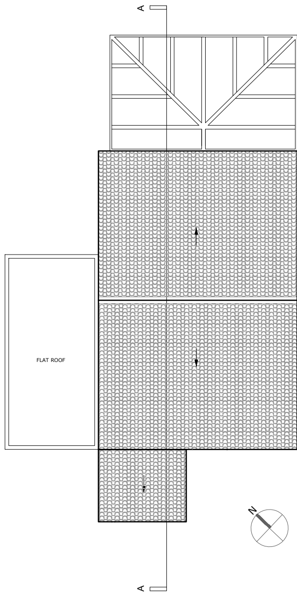
PRE - EXISTING ROOF PLAN
