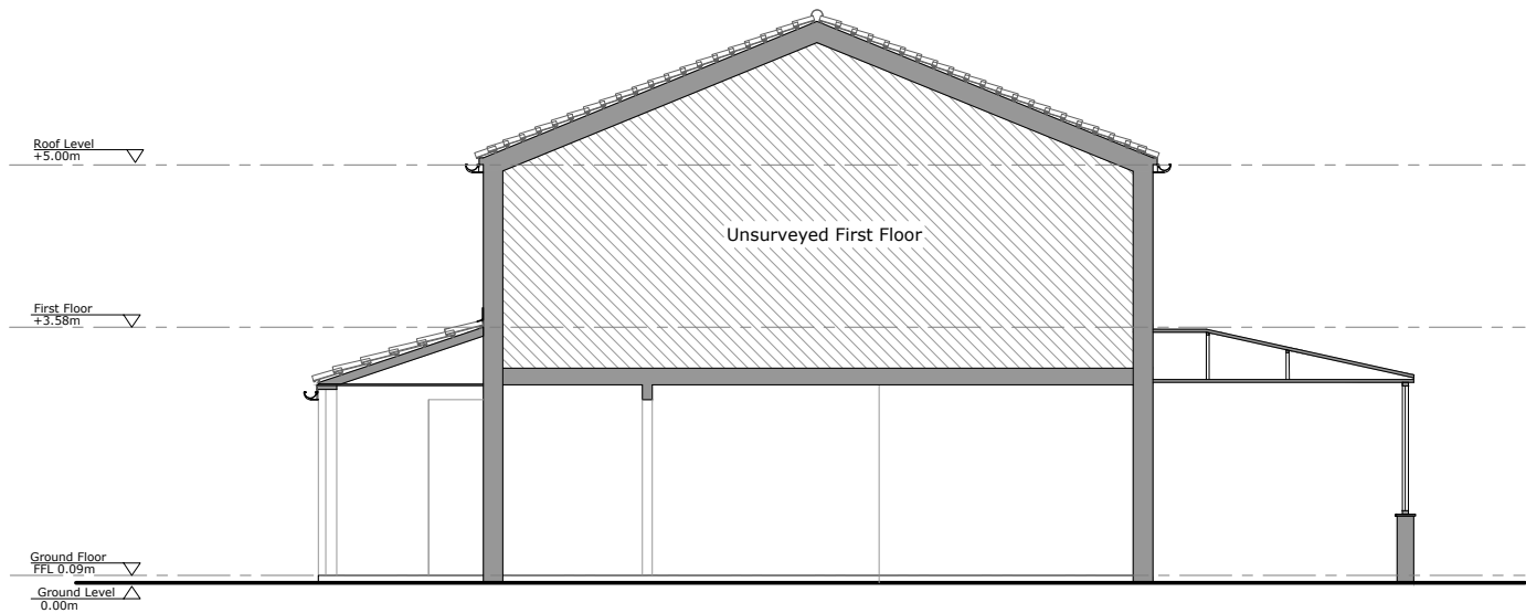
PRE - EXISTING SECTION A-A
