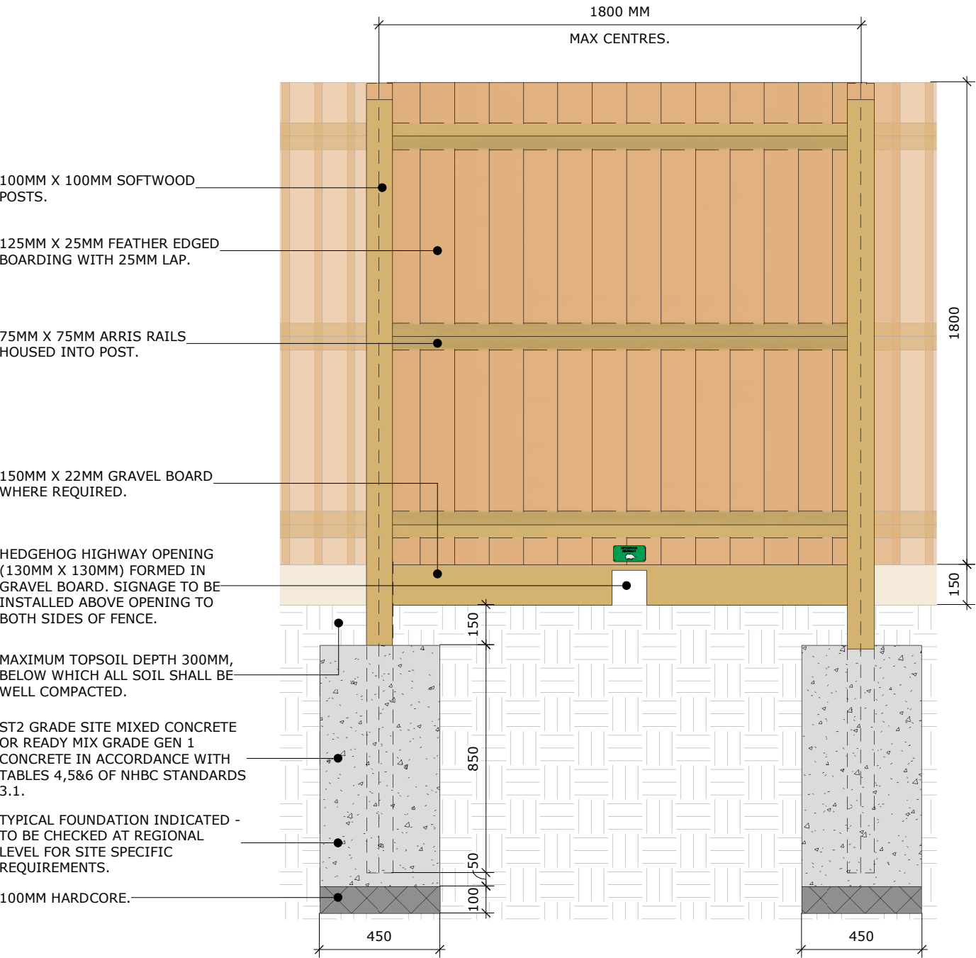
CLOSE BOARD FENCE - ELEVATION
