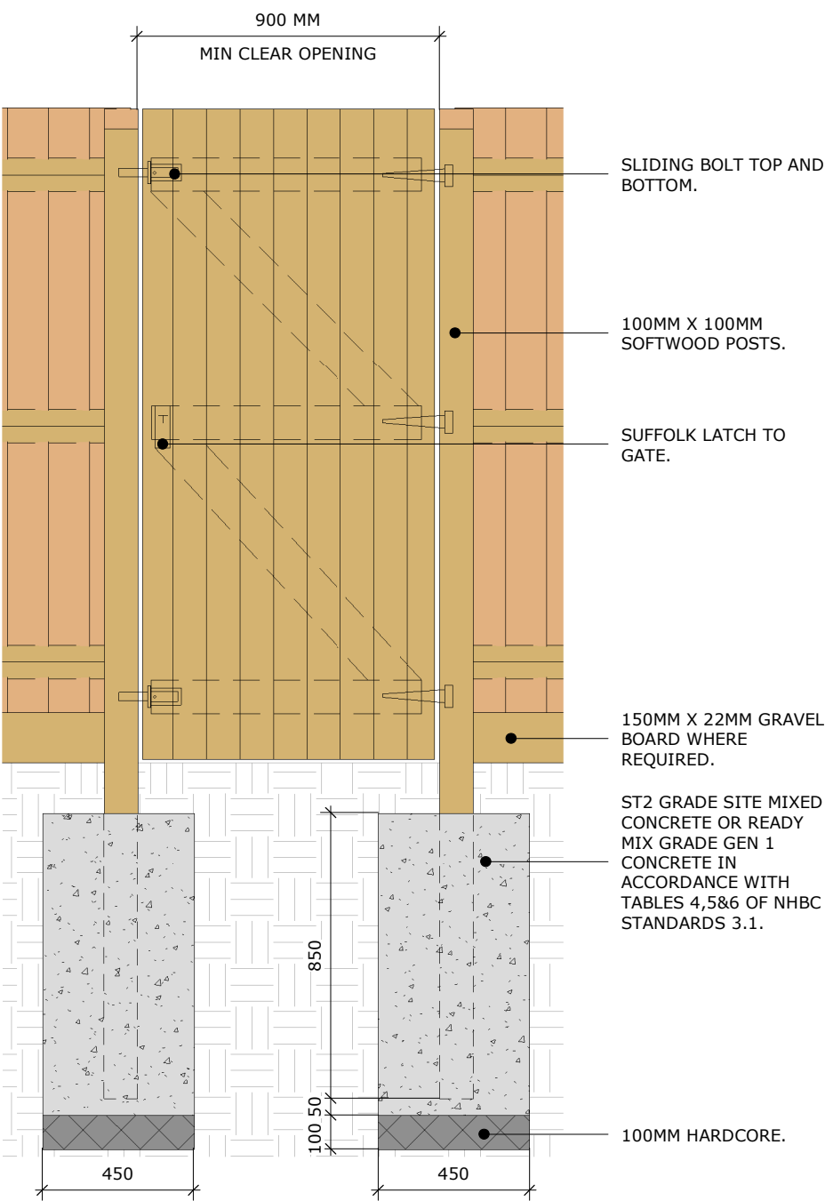
GATE ELEVATION
