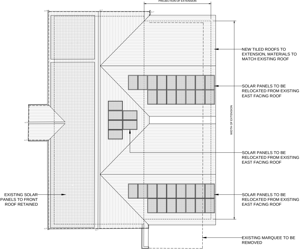
ROOF PLAN
