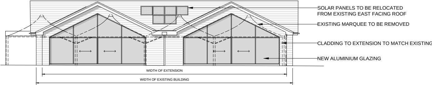
EAST ELEVATION
