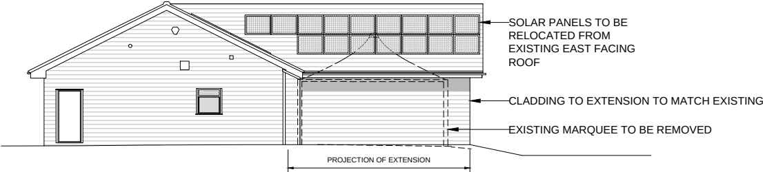
SOUTH ELEVATION
