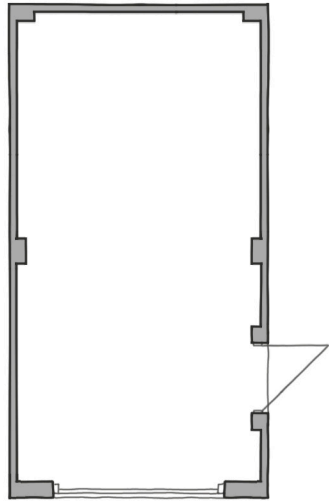
GARAGE FLOOR PLAN
