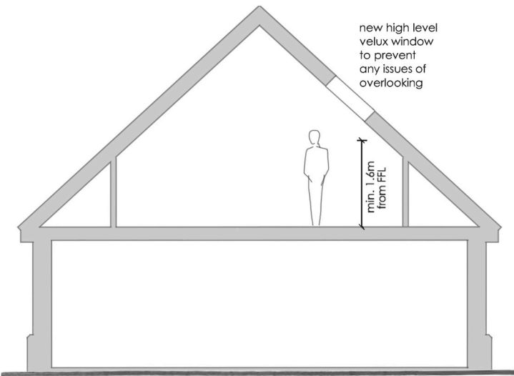
PROPOSED SECTION - typical velux window height
