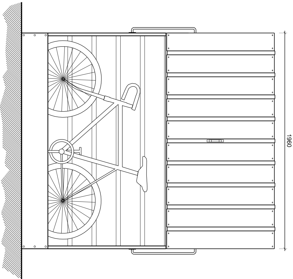
Front Elevation - Open
