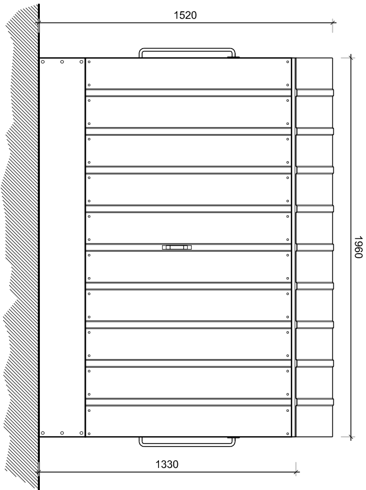
Front Elevation - Closed
