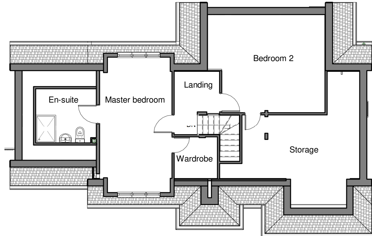
1 EXISTING FIRST FLOOR PLAN 1 : 100
