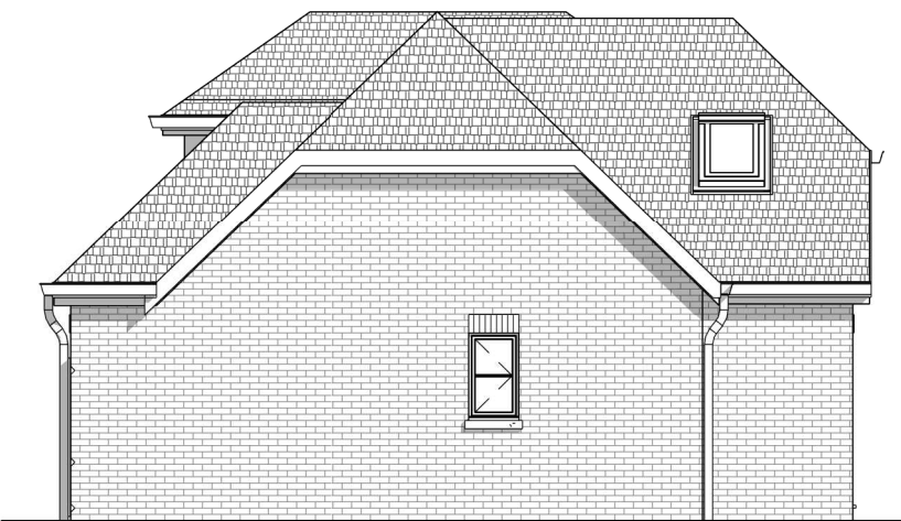
4 EXISTING SIDE ELEVATION
