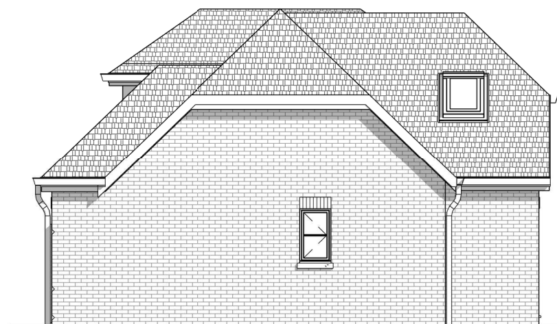
4 PROPOSED SIDE ELEVATION 1 : 100
