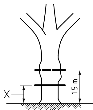
d) Measurement of stem with irregular swelling made at the narrowest point below the swelling
