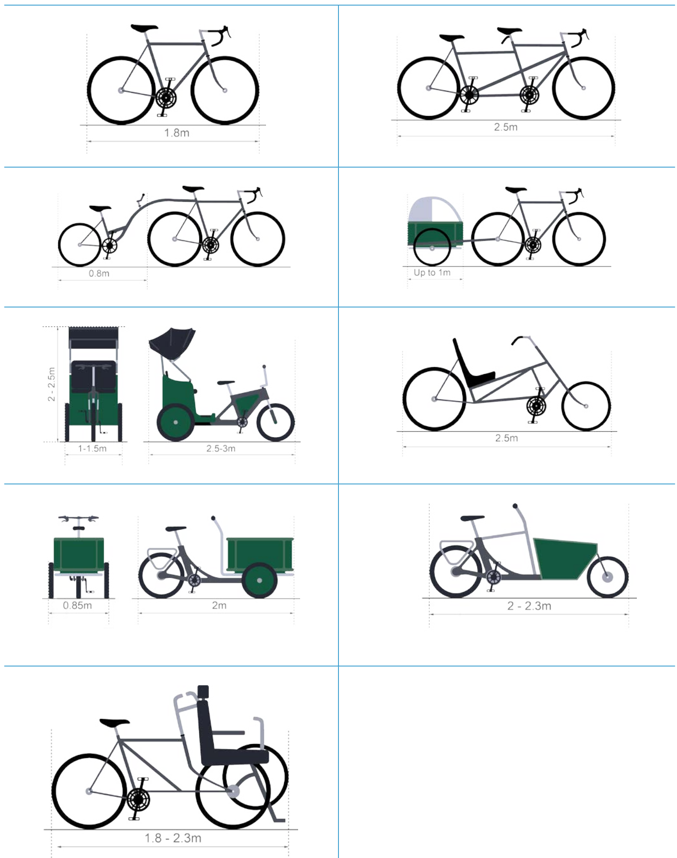
Figure 5.2: Typical dimensions of cycles
