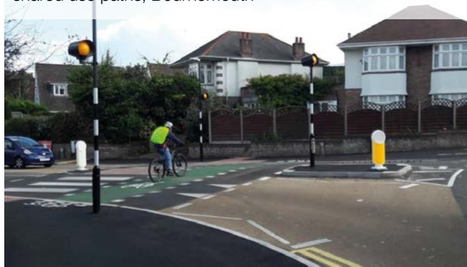
Figure 10.38: Roundabout with parallel crossings and shared use paths, Bournemouth
