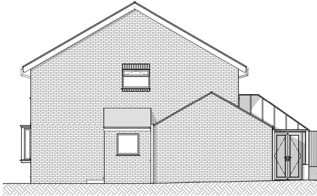
Existing Elevation - North-East
