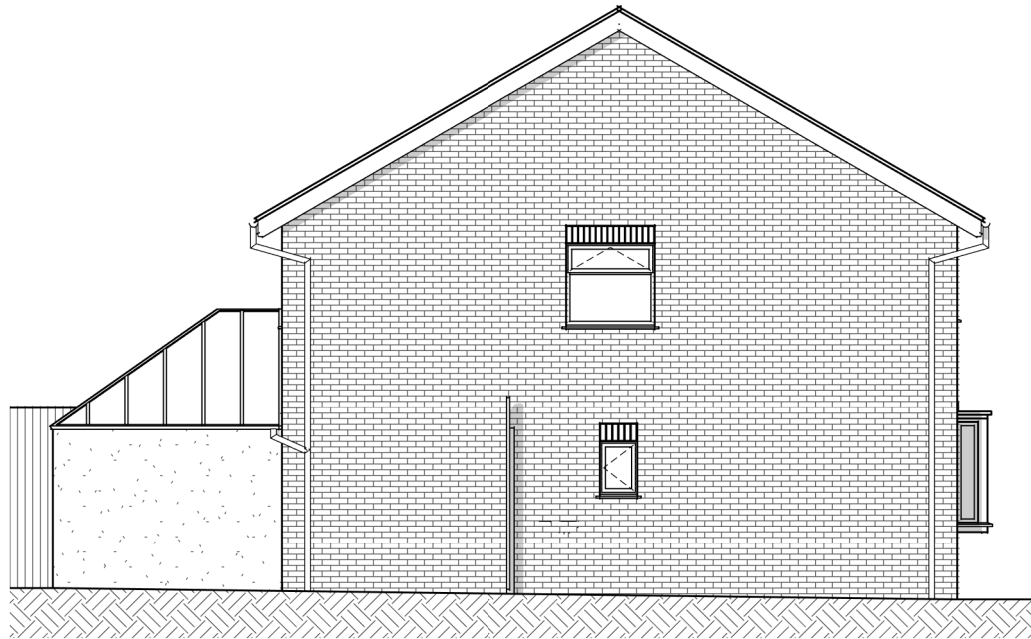
Existing Elevation - South-West
