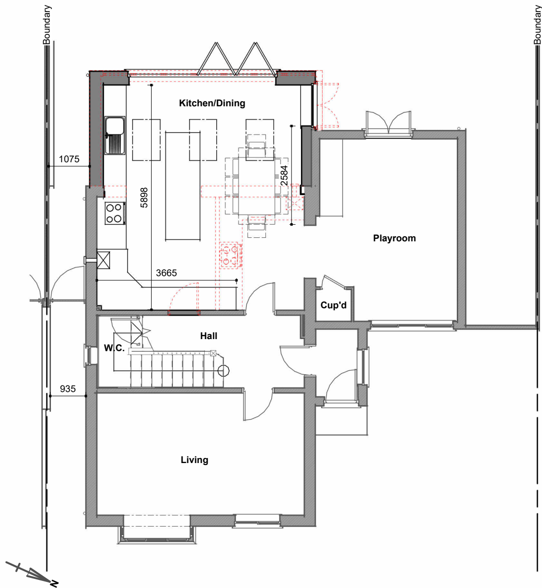
Proposed Ground Level Plan
