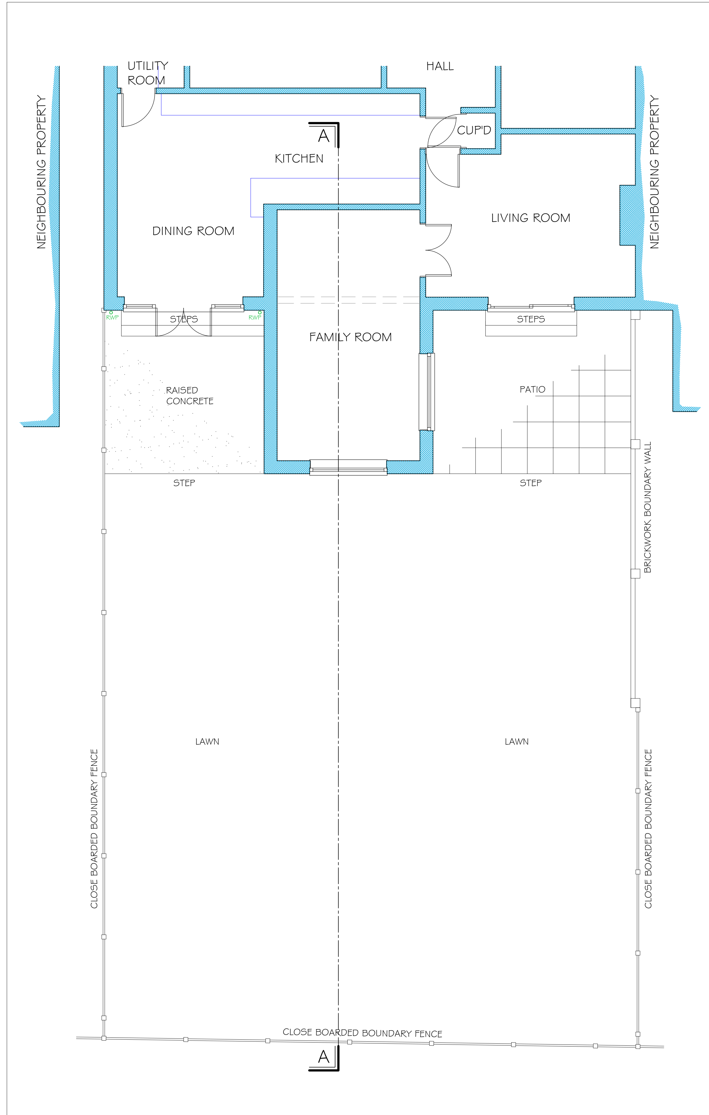
FORMER FLOOR PLAN & GARDEN LAYOUT 1:50
