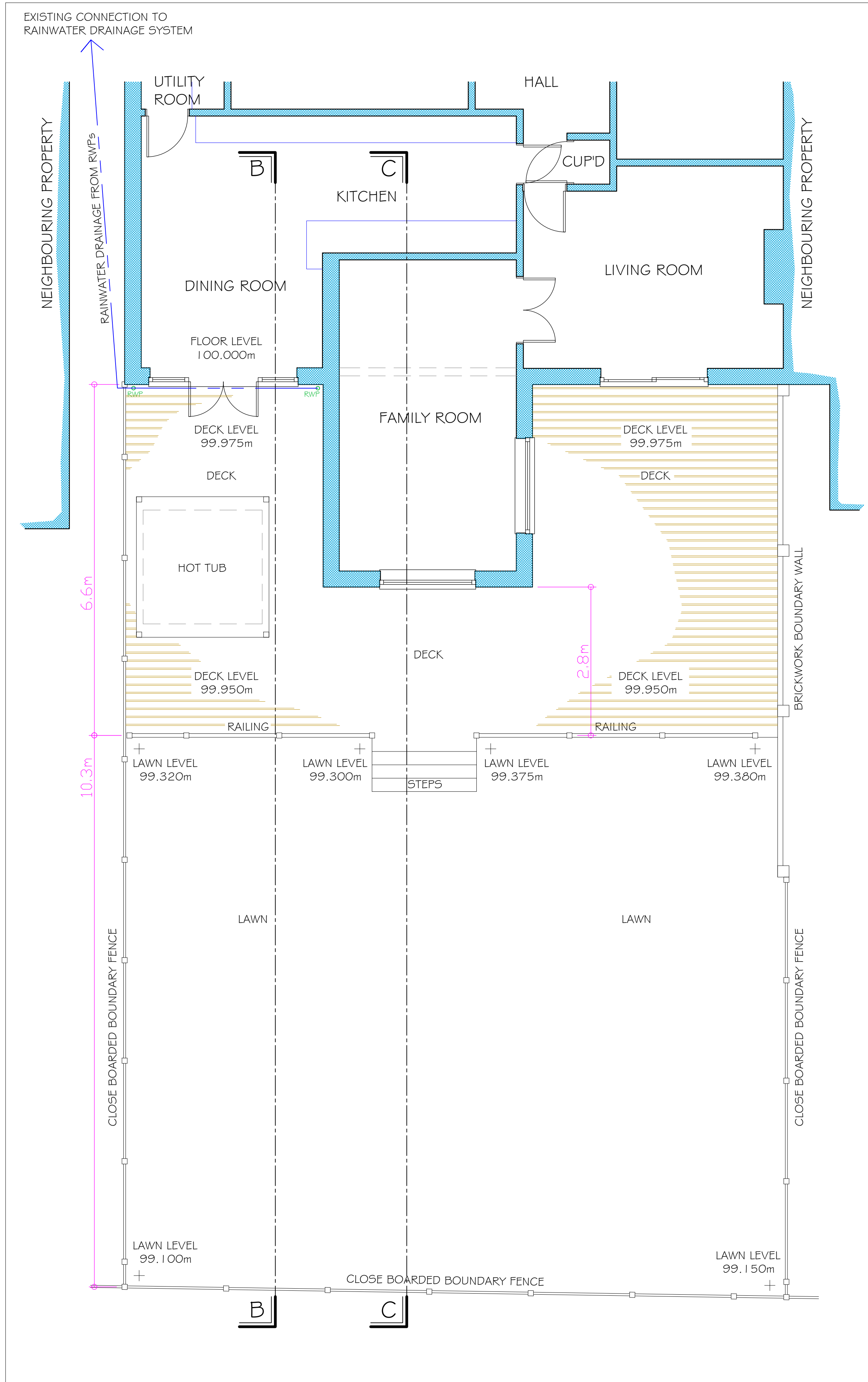
CURRENT FLOOR PLAN & GARDEN LAYOUT 1:50
