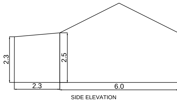
PROPOSED ELEVATION
