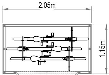
Shed Plan Scale - 1@50 @A1
