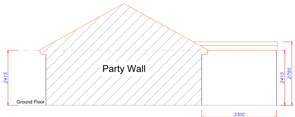
Proposed Right Elevation
