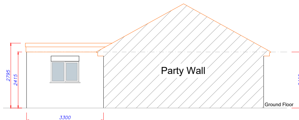
Proposed Left Elevation
