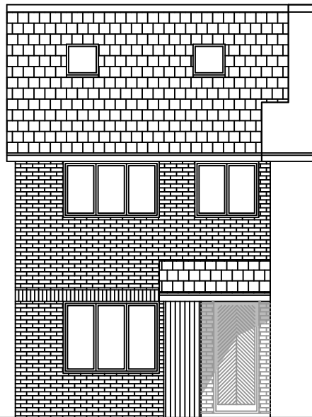
Front 1:100
