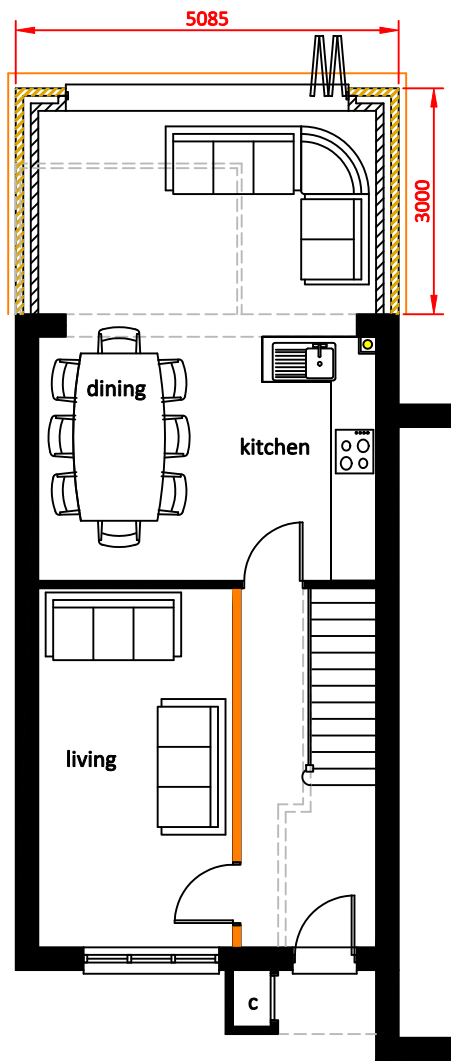
Ground 1:100
