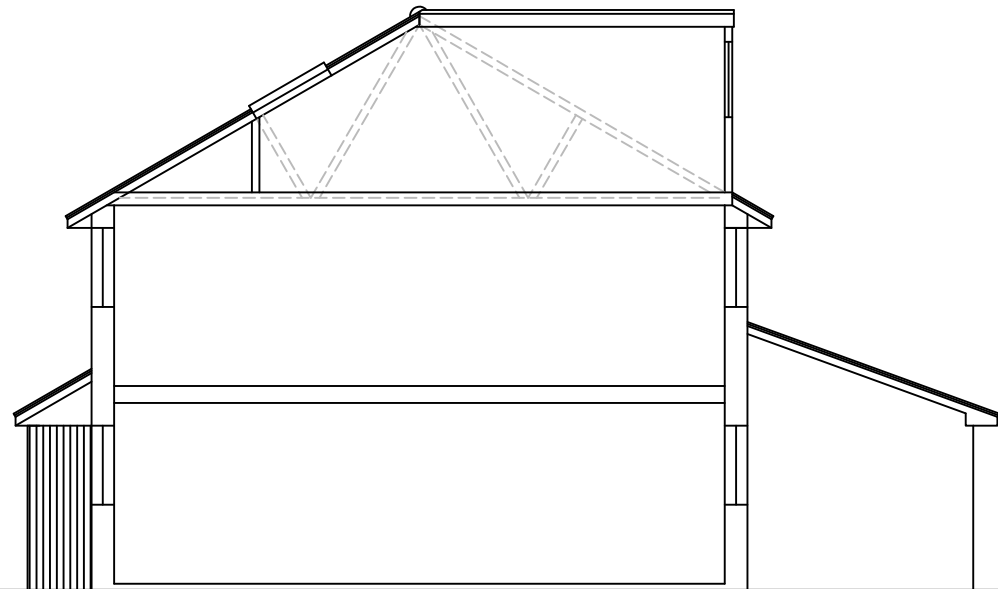
Section
