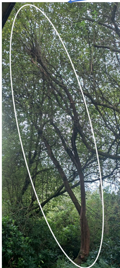
Tree 2
