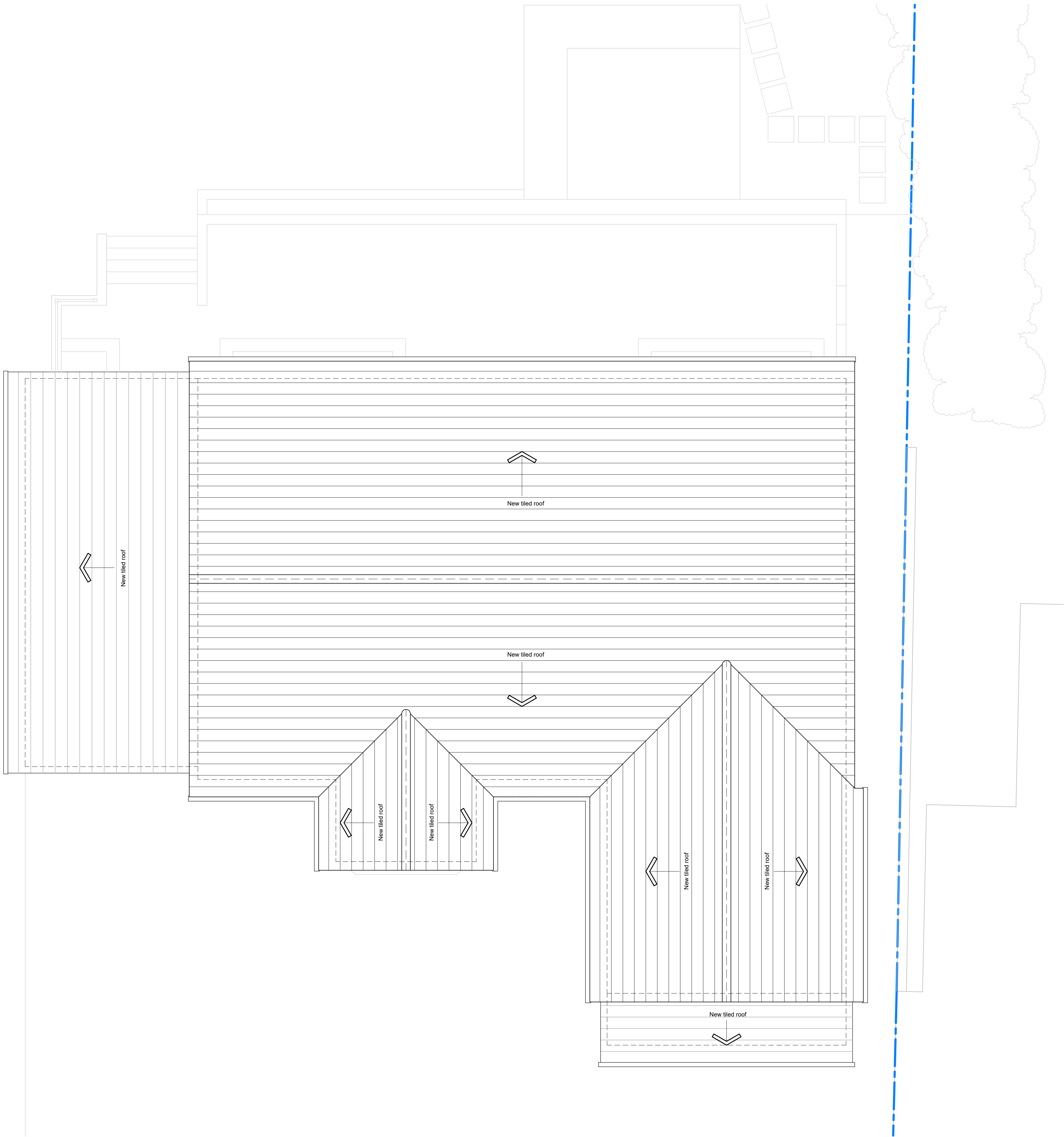
PROPOSED ROOF PLAN
