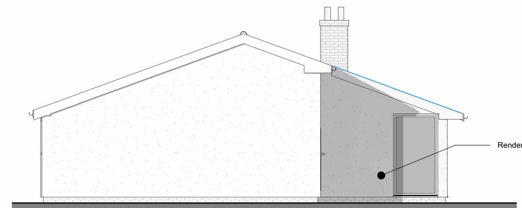
Side 2 Elevation
