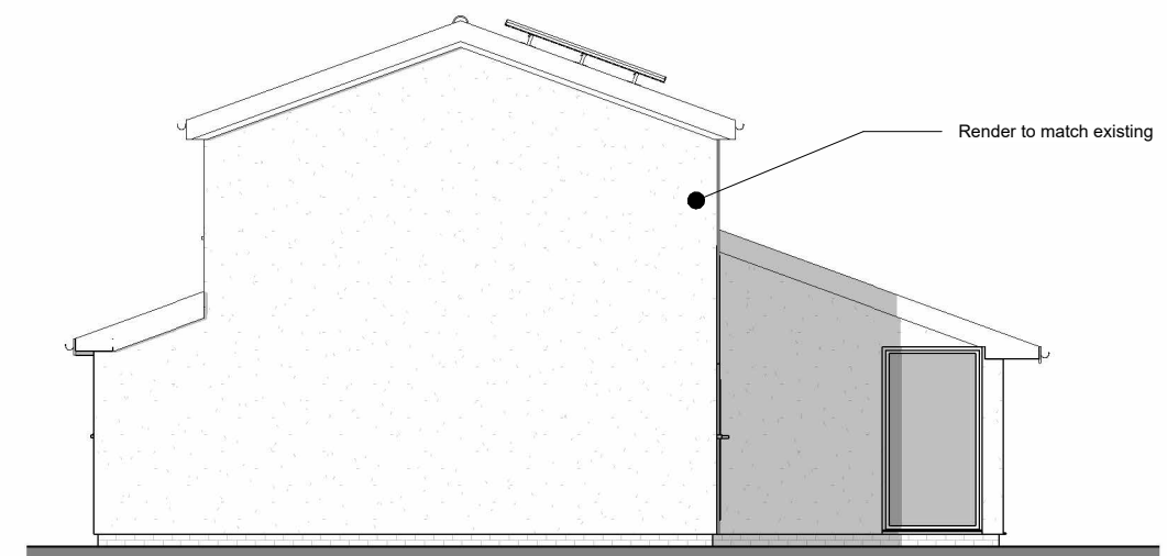
Side 2 Elevation
