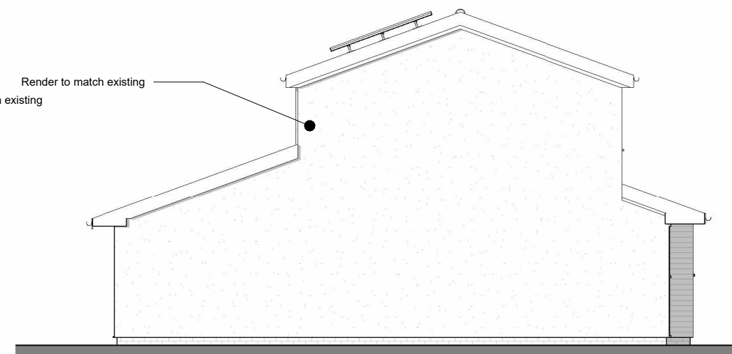
Side 1 Elevation
